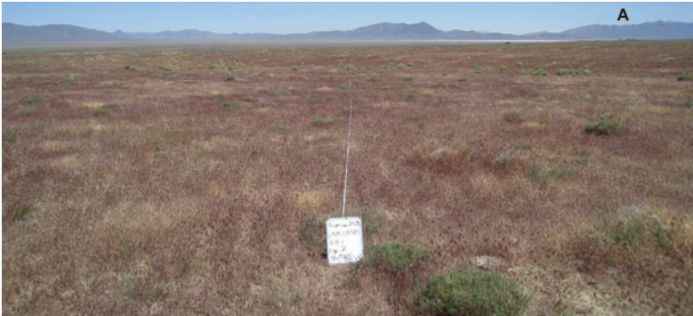
Figure 12. Nine-year post wildfire (2002) response for adjacent (A) seeded and (B) unseeded communities. Ecological site is a warm-mesic/dry-aridic Wyoming big sagebrush/Indian ricegrass-Sandberg bluegrass type, at an elevation of 5,000 ft southeast of Gerlach Nevada. Native herbaceous vegetation prior to the burn was likely severely depleted to absent and the presence of a sagebrush canopy was unknown. Soil temperature + moisture score = 9, total score 9-12. This site has low suitability for seeding and low resilience to disturbance. The treated site (A) was drill seeded to native grasses in the fall following the fire and (B) was not seeded. Cover in the treated site (A) is 0% native deep-rooted perennial grasses, 61% cheatgrass, 3.3% native shrub cover and 6% non-native shrub cover. Cover in the untreated site (B) is 0% deep rooted perennial grasses, 89% cheatgrass, 6.7% native shrub cover and 0% non-native shrub cover.
