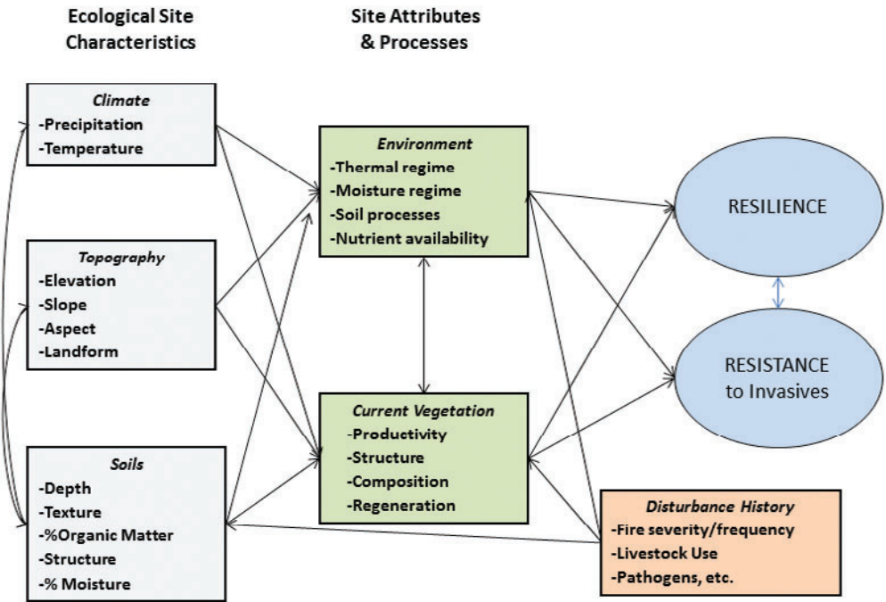
Figure 3. A conceptual model that illustrates the factors that influence resilience to treatment and resistance to invasive species. Ecological site characteristics or environmental factors are the primary factors that influence soil temperature/moisture regimes and potential vegetation. The regimes are identified in soil maps as mesic (warm), frigid (cool), cryic (cold), aridic (dry), and xeric (moist). Potential vegetation + disturbance history + time since disturbance or treatment = current vegetation. If all of the ecological site characteristics are favorable for treatment and the site attributes and processes are all functioning within the natural range of variability then levels of resilience to treatment application and resistance to invasive species are near potential for that site. However, if the site is not at potential because one or more components are below potential or missing, for example, perennial grasses are severely depleted or invasive annual grasses are abundant, resilience to disturbance and/or resistance to invasive annual grasses will be lower than potential (adapted from Chambers and others 2014a).
