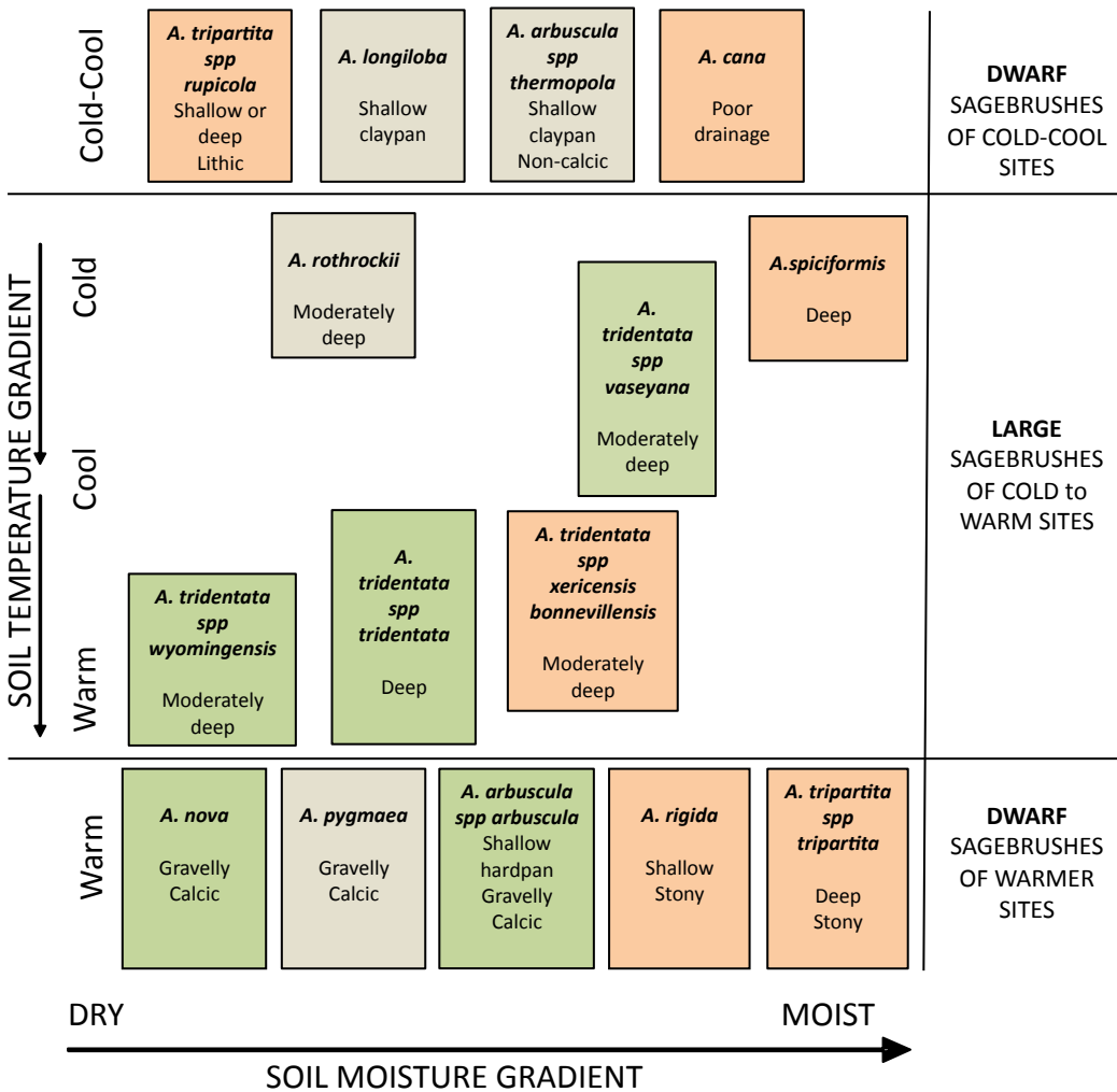
Figure 5. Major sagebrush taxa in the Great Basin and Columbia River Plateau positioned along gradients of soil temperature and soil moisture (adapted from Robertson and others 1966; McArthur 1983; West 1983; West and Young 2000; Rosentreter 2005; Schultz 2009, 2013). Key soil characteristics associated with each species are shown under the species name. Relative abundance of the sagebrush species and subspecies in the Great Basin and Columbia River Plateau is color coded: grey = scarce, orange = common, and green = dominant.
