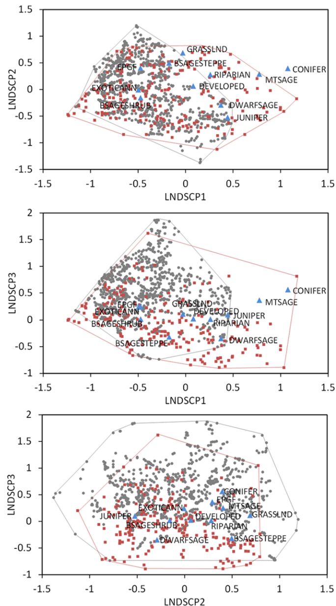
Fig. A2. NMS biplots, each showing 211 plots sampled for sage-grouse occupancy and habitat (red) and 826 plots associated with ESR projects (gray) in two-dimensional landcover space. Plots closer together in ordination space have more similar landscape compositions (within a 5 km radius) to one another. Centroids for certain landcover types are shown (blue triangles) and are labeled as in Table A1. The remaining landcover types were used in the NMS analysis, but were omitted from these figures for clarity. As expected (based on our ESR site selection and stratification approach and the location of these plots within burned landscapes), ESR plots predominantly occupy a subset (albeit a large subset) of the landscapes where sage-grouse occupancy and habitat were assessed in randomly placed plots. Ninety-four percent of ESR plots fall within the ordination space occupied by random plots. Thus, landscapes similar to those of our ESR plots are well represented in the sage-grouse occupancy and habitat data. Consequently, occupancy rates in these randomly located plots should provide inference for occupancy rates in ESR plots.
